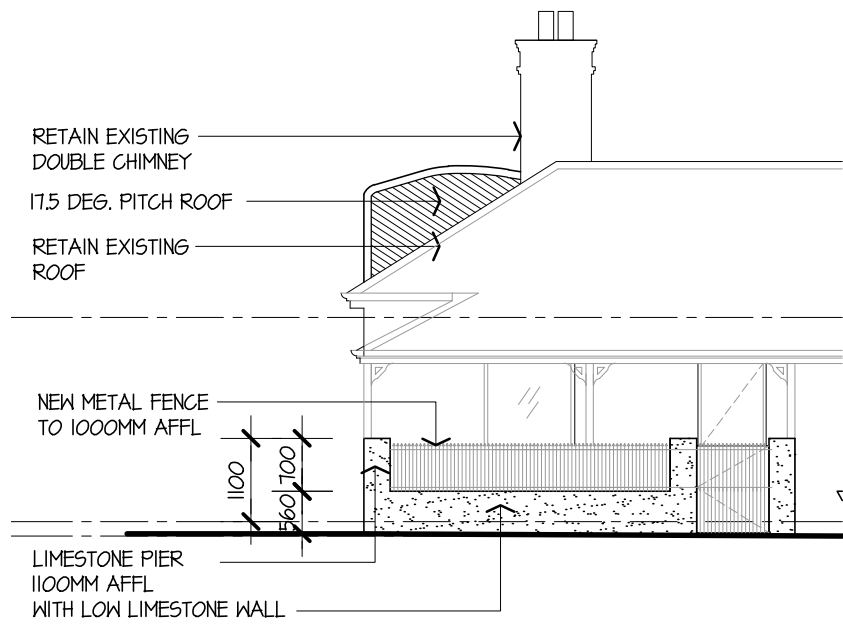
NORTH ELEVATION
